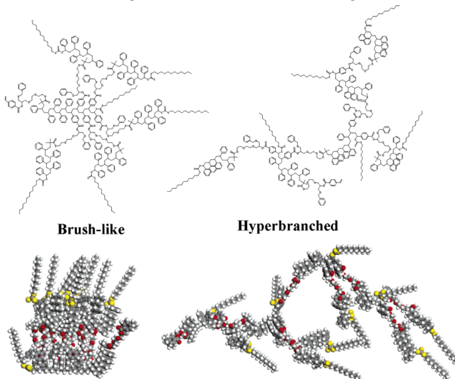
Scheme 4. Chemical Structure and Corresponded Molecular Models of Two Possible Expected Architectures of the Polymer P3
