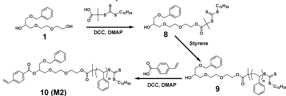
Scheme 2. Synthesis of the Macroinimer M2
