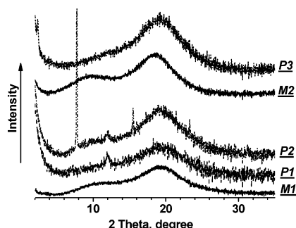
Figure 8. X-ray diffraction data of the macroinimers and corresponded hyperbranched polymers. Sharp peaks are due to the presence of unremovable organic impurities in polymers.
