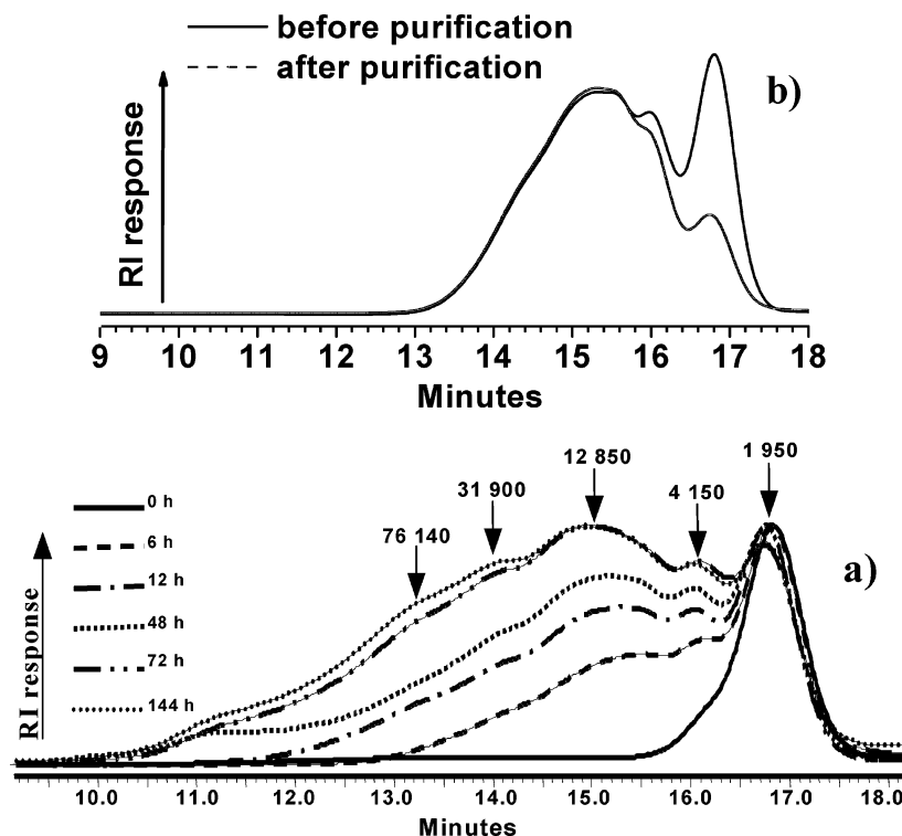
Figure 3. GPC traces of the polymerization of M1 in bulk at 125 °C (a) and hyperbranched polymer P2 before and after purification (b). Peak values were calculated using PS calibration curve.
